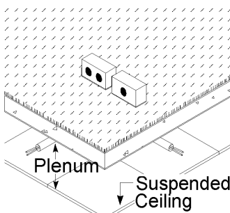
Fig. 23 Poke-through distribution
