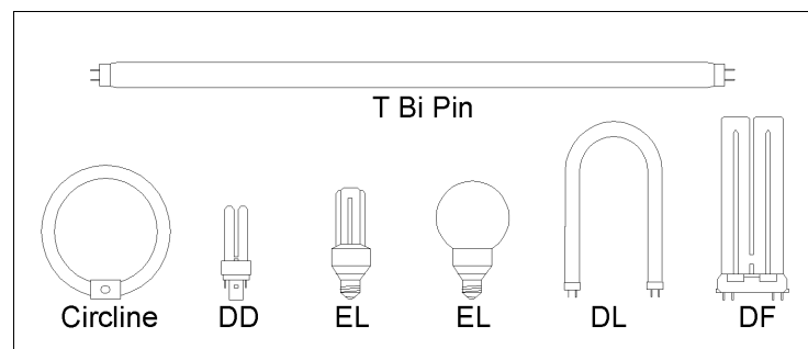
Fig. 26 Fluorescent lamp types
